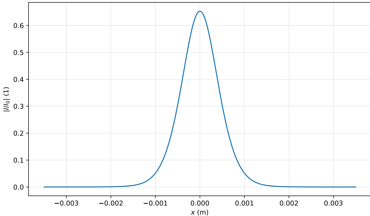
Intensity profile I(x, y = 0, z = 3.105m)/I_0 , P_{in}=0.6P_{cr} , artificial time
